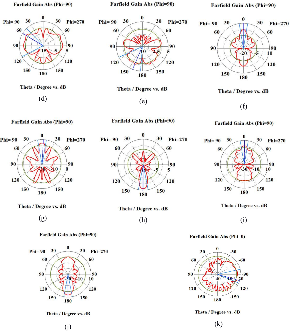
Figure 5 Radiation pattern of optimized MPA at various frequencies (a) at 7.76GHz (b) at 11GHz (c) at 18.128GHz (d) at 30.8GHz (e) at 37.84GHz (f) at 60.368GHz (g) at 74.064GHz (h) at 79.765GHz (i) at 85.456GHz (j) at 92.88GHz (k) at 98GHz
