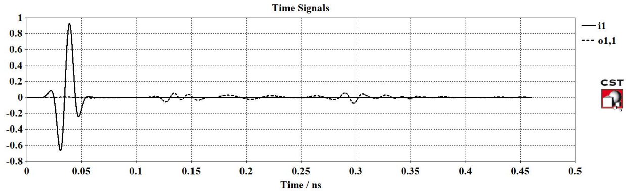
Figure 2 Transient behavior of SWB MPA
