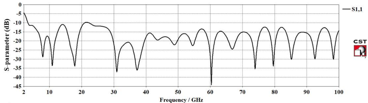
Figure 3 S_{11} response of optimized MPA
