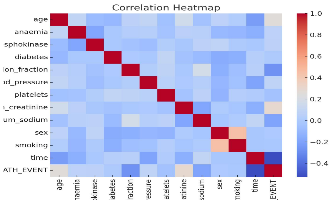
Figure 3: Correlation Heatmap
